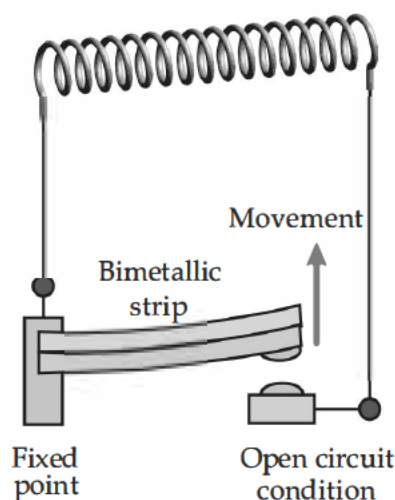
Fig 9.10 Bimetallic Thermostat
