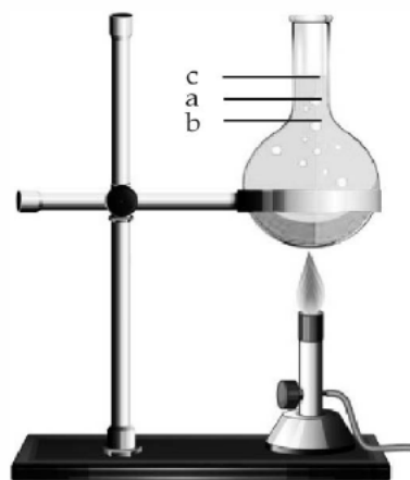
Fig 9.14 Real and Apparent expansion of liquids
